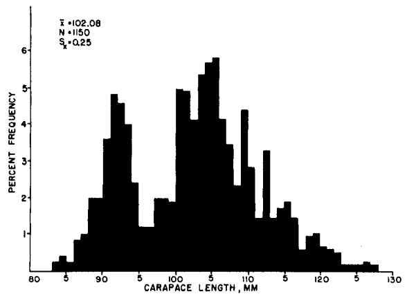
FIGURE 10.—Length-frequency distribution of native Maine berried females, 1966 through 1970.
